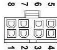
8pin Connector
